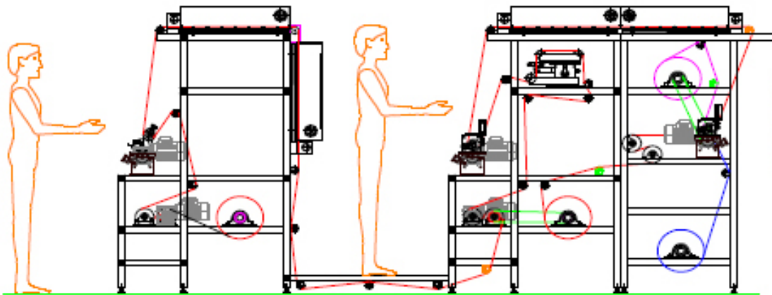
Left and below is an illustration of a typical multi drive, inline 2 colour converting machine.
